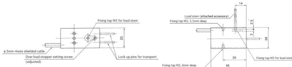
Model and Capacity / Dimension / etc. (unit : mm)
