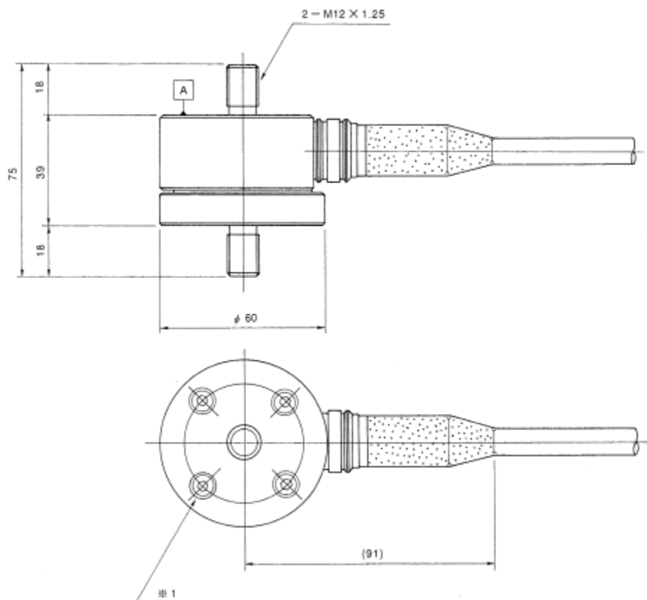
Model and Capacity / Dimension / etc. (unit : mm)
