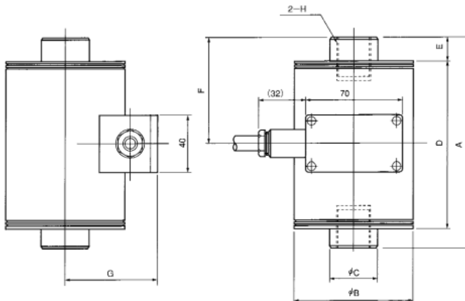
Model and Capacity / Dimension / etc. (unit : mm)
